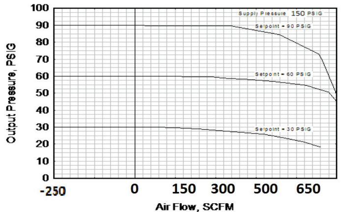
Flow Characteristics T9080-4078N4FNT Pressure Controller
