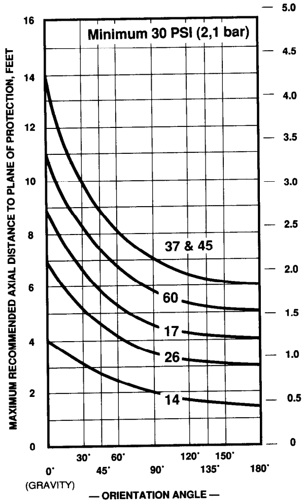
FIGURE C-2 — WATER DISTRIBUTION DESIGN DATA — MAXIMUM RECOMMENDED AXIAL DISTANCE TO PLANE OF PROTECTION
