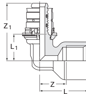
MLC-S Press Female 90° Elbow
