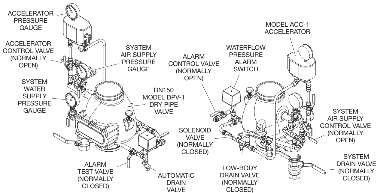
FIGURE 10 (2 OF 2) DN150 MODEL DPV-1 PREACTION TYPE B VALVE TRIM ASSEMBLY COMPONENTS
