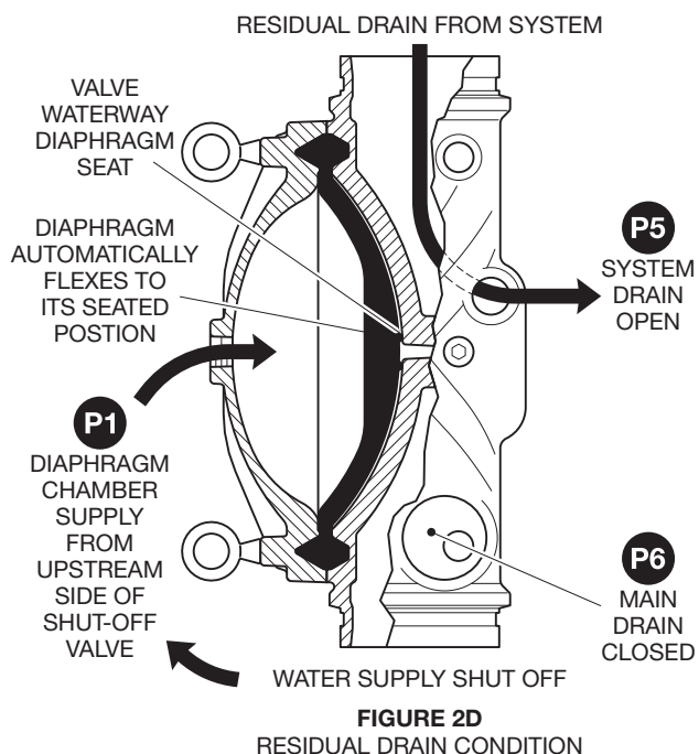
FIGURE 2 DV-5A VALVE OPERATION, DELUGE REMOTE-RESETTING, PRESSURE-REDUCING SYSTEMS
