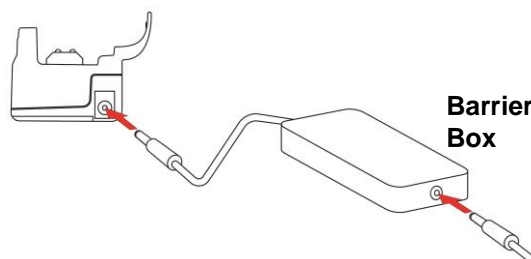
ATEX/IECEx: Barrier Box Between power supply and Travel Charger.
