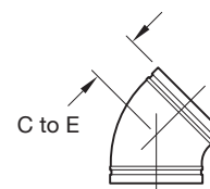
FIGURE 501 CAST 45° ELBOW
