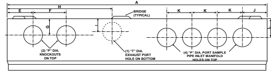
Detector Mounting Box
