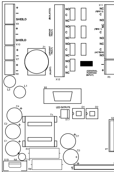
Detector Termination Card 7 Relay Version
