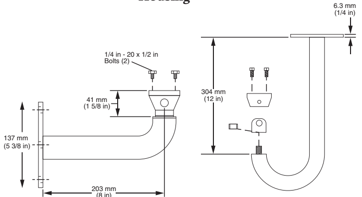
Wall Mount Side View ADCHMTWALL
