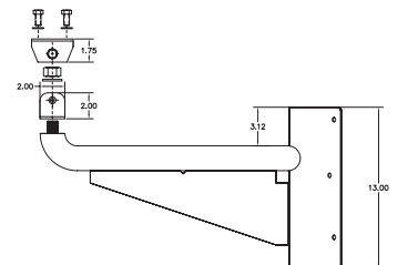
Corner Mount Side View ADCHMTCRNR
